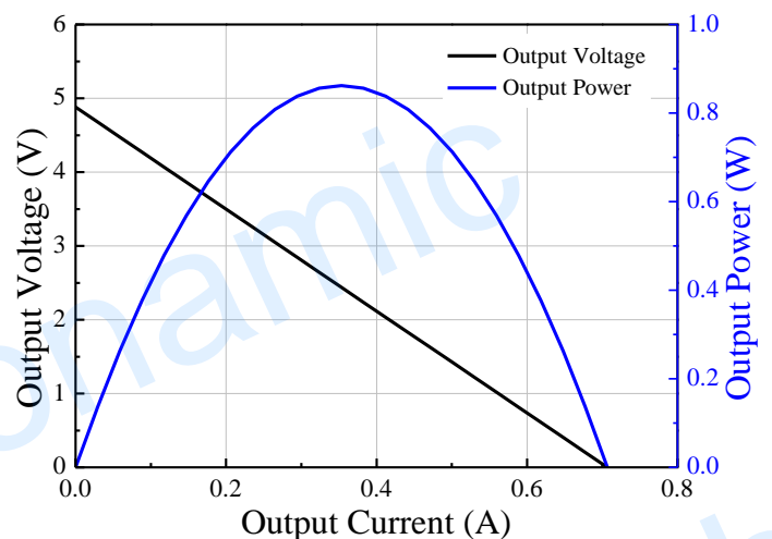
The chart for output voltage and output power Vs output current under T_h = 230^\circ\text{C} and T_c = 50^\circ\text{C}
